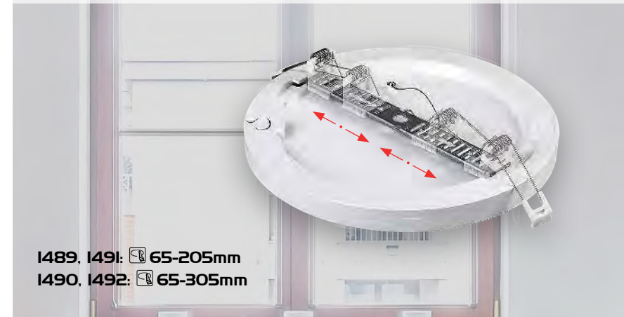
1491 LED / 18W (1500lm, 4000K) incl. IP20 • white • 8m, 130° 65-205mm • 70mm
